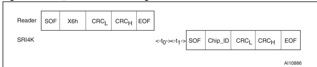
Figure 31. Slot_marker frame exchange between reader and SRI4K
